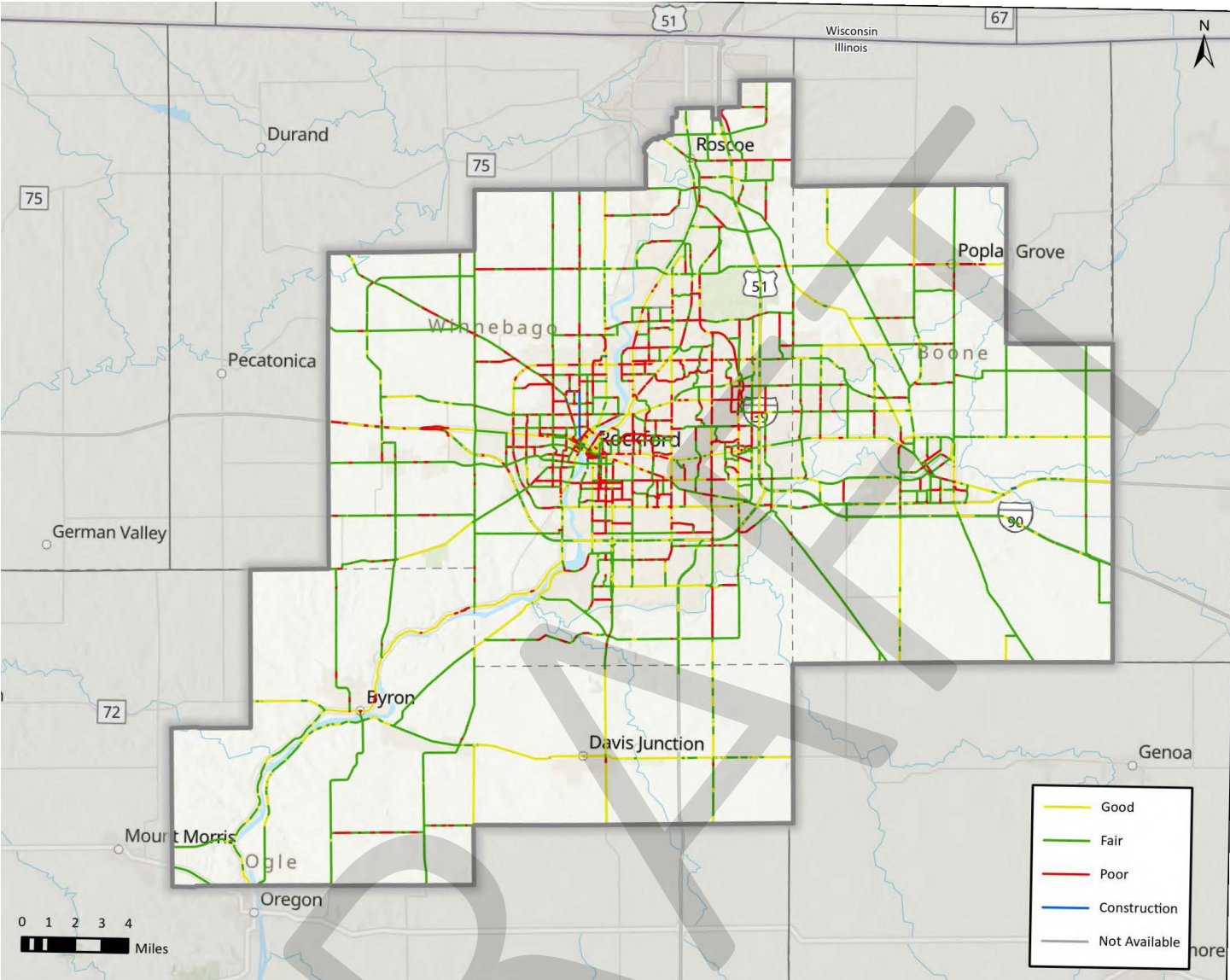
Figure 4-2: MPA Pavement Condition
